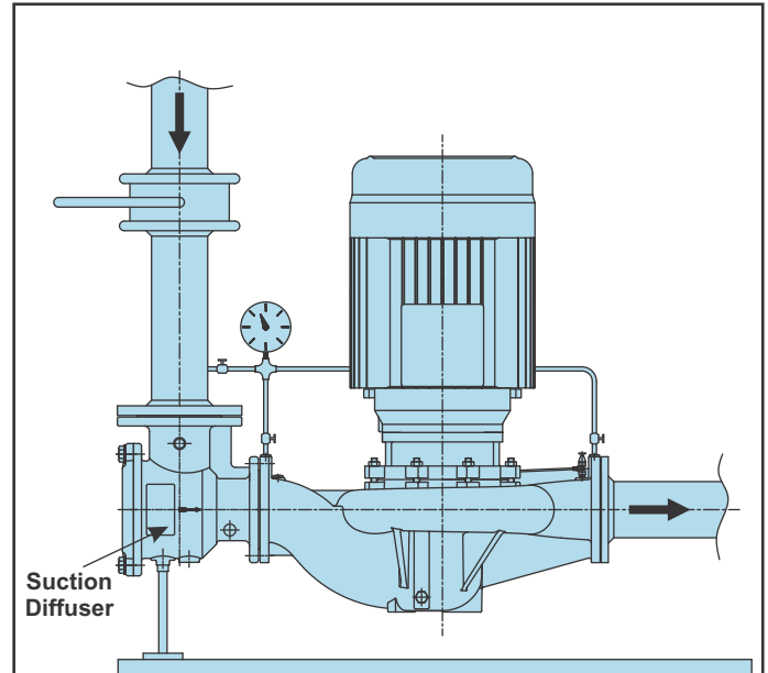
VERTICAL IN-LINE PUMP
