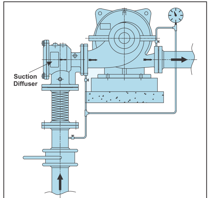
HORIZONTAL SPLIT CASE PUMP
