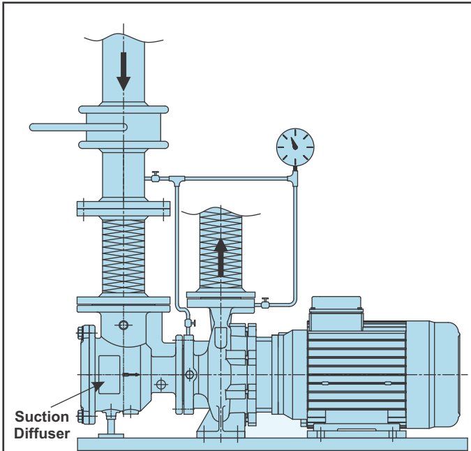
END-SUCTION CLOSE COUPLED MOTOR PUMP
